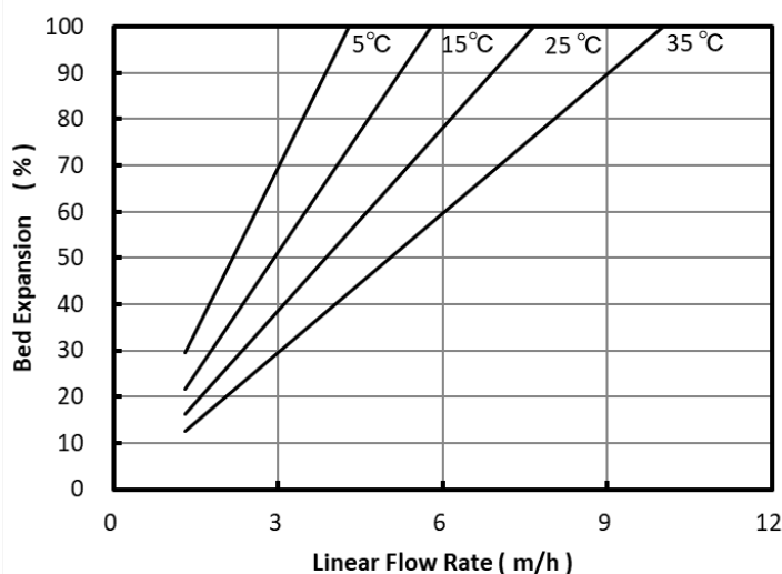
Fig. 2 Bed Expansion of JA310C
