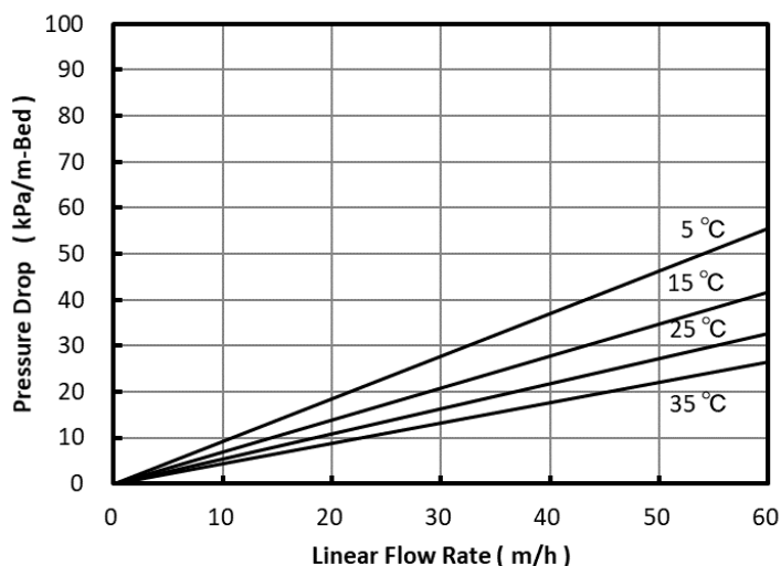
Fig. 1 Pressure Drop of JA310C
